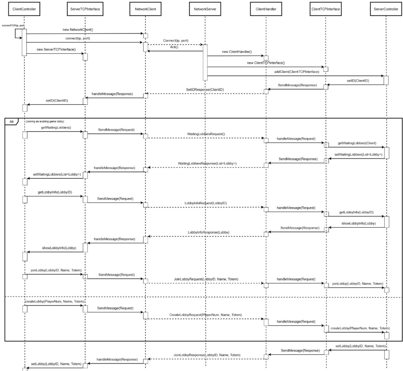
Game access TCP sequence diagram
